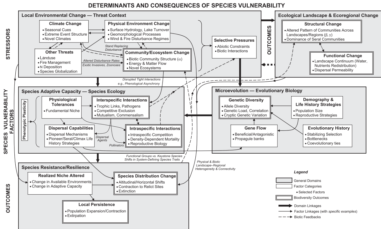
Figure 1 Determinants and consequences of species vulnerability. The figure is broadly organized into domains of stressors (climate and other anthropogenic environmental changes, top left panel), species-level vulnerability factors (which limit or support a species' adaptive capacity, middle panels), and outcomes. Factors that set a species' vulnerability are its current adaptive capacity (middle left panel) and microevolutionary shifts in this capacity (middle right panel). Outcomes of these vulnerabilities include species persistence and range changes (bottom panel), altered landscape and regional ecological heterogeneity (top right panel), and changes to genetic diversity, community structure, and the complexity of ecosystem interactions – all of which are elements of biodiversity (double-bordered boxes). Selected factors (bulleted items) give examples for factor categories, and factor linkages and feedbacks (narrow-lined arrows) illustrate interactions; not all possible factors and linkages are shown. With respect to local and regional/landscape community structure, symbols \alpha , \beta , and \gamma refer to Whittaker's (1960) levels of species diversity, where \alpha = site (sample) species diversity, \gamma = regional total diversity, and \beta = among-sample heterogeneity in species diversity across the region.
