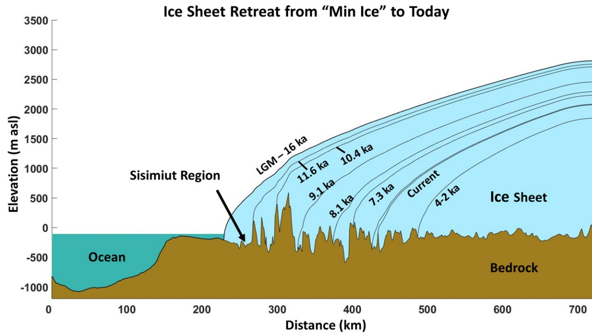
Fig 1. Cross section of crustal rebound model showing "max ice" and "min ice" LGM position and retreat history.
