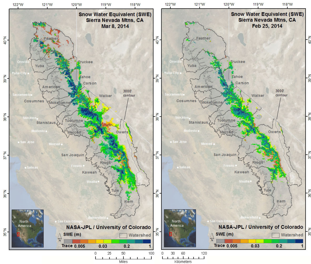
Figure 1. RT simulated SWE amounts for Mar 8, 2014 are shown on the left and for Feb 25, 2014 are shown on the right. SWE depths have increased at all elevations and snow extent has increased since the last report.
