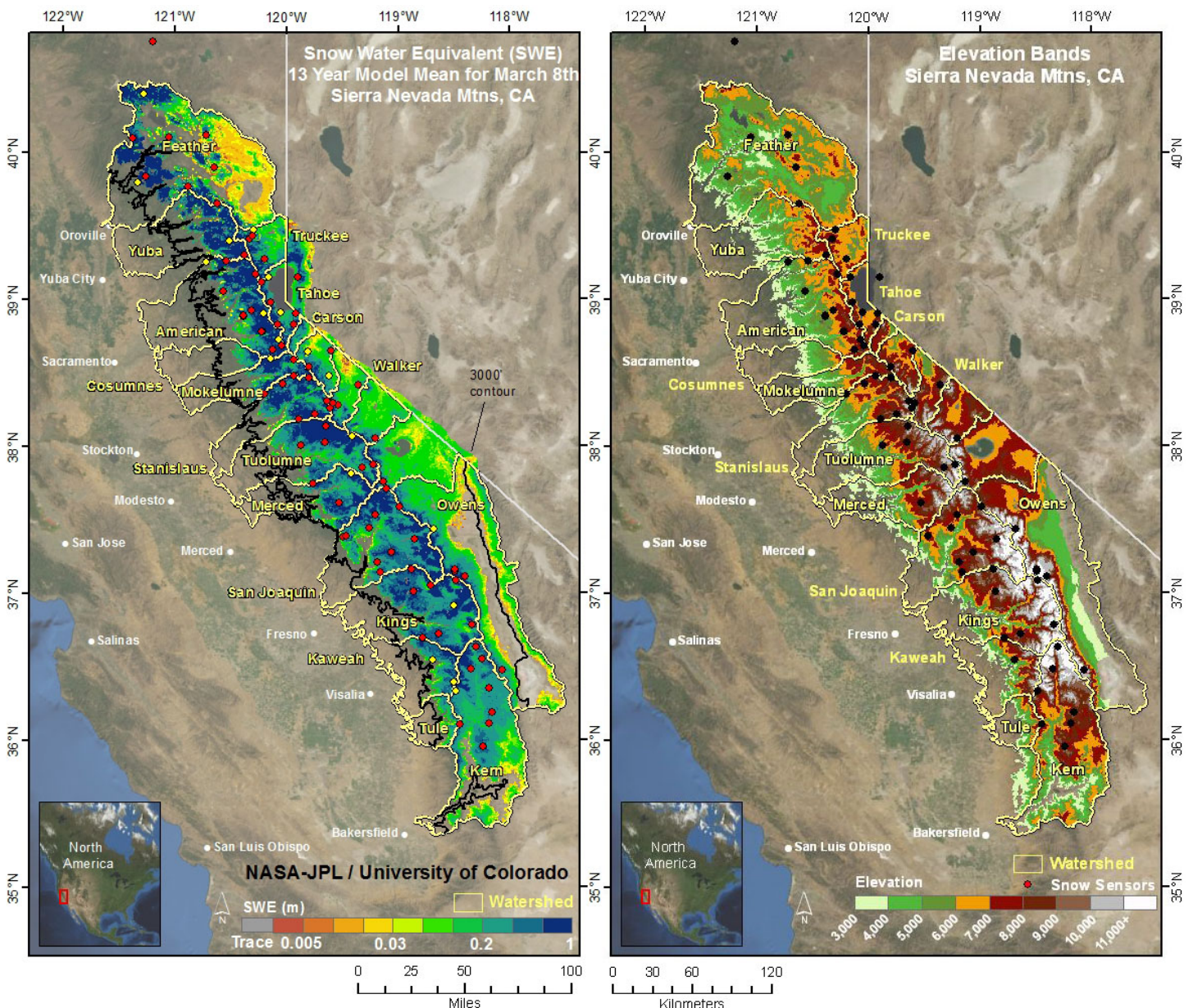
Figure 3. 13 year modeled average SWE for March 8 th on the left with snow sensors shown in yellow that recorded no snow (see discussion above for an explanation) and in red for sensors that recorded snow on March 8, 2014; and a banded elevation map on the right.
