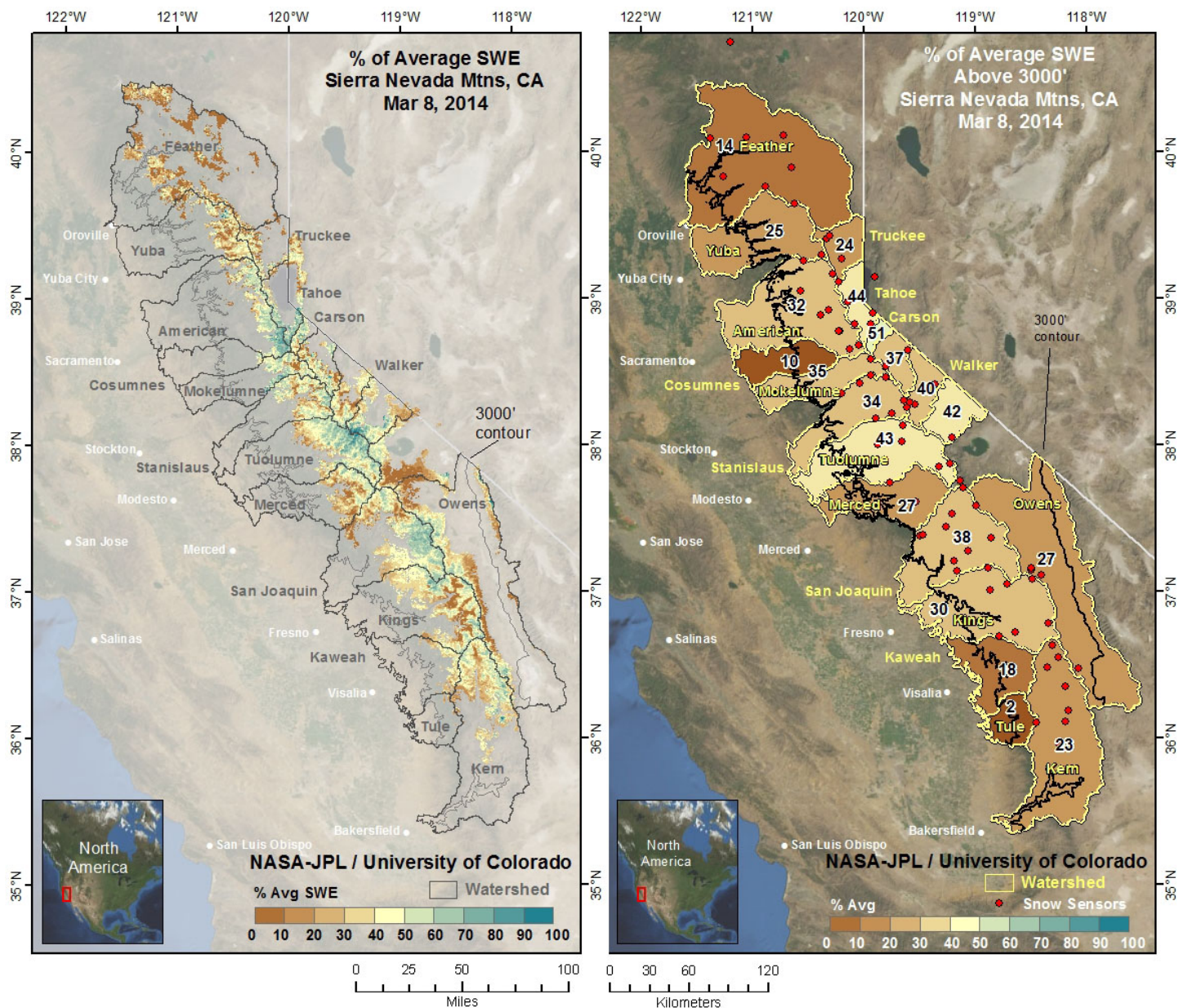
Figure 2. Percent of average RT simulated SWE for March 8, 2014 for the entire Sierra (on left) and by watershed (on right). Watershed percentages are calculated for all model pixels above 3000' (shown as gray line on left map). SWE snow sensors that had snow on March 8, 2014 have been added to the map on the right.
