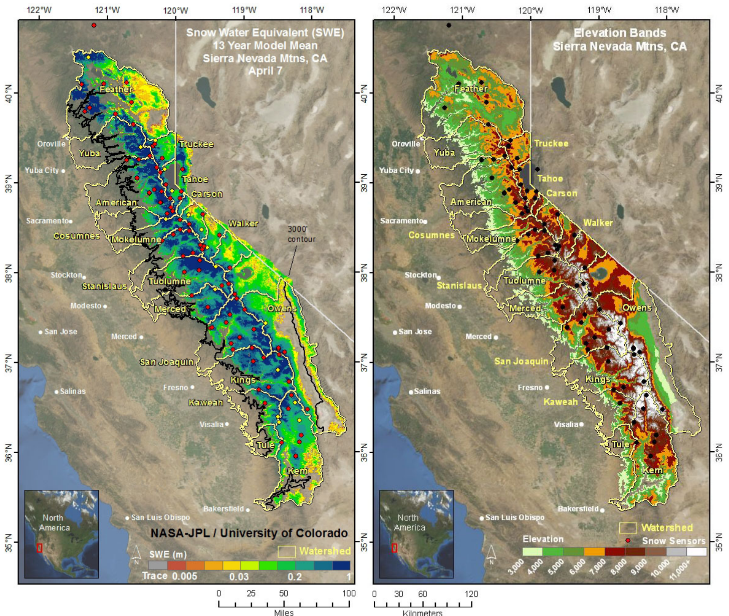
Figure 3. 13 year modeled average SWE for April 7 th on the left with snow sensors shown in yellow that recorded no snow (see discussion above for an explanation) and in red for sensors that recorded snow on April 7, 2014; and a banded elevation map on the right.
