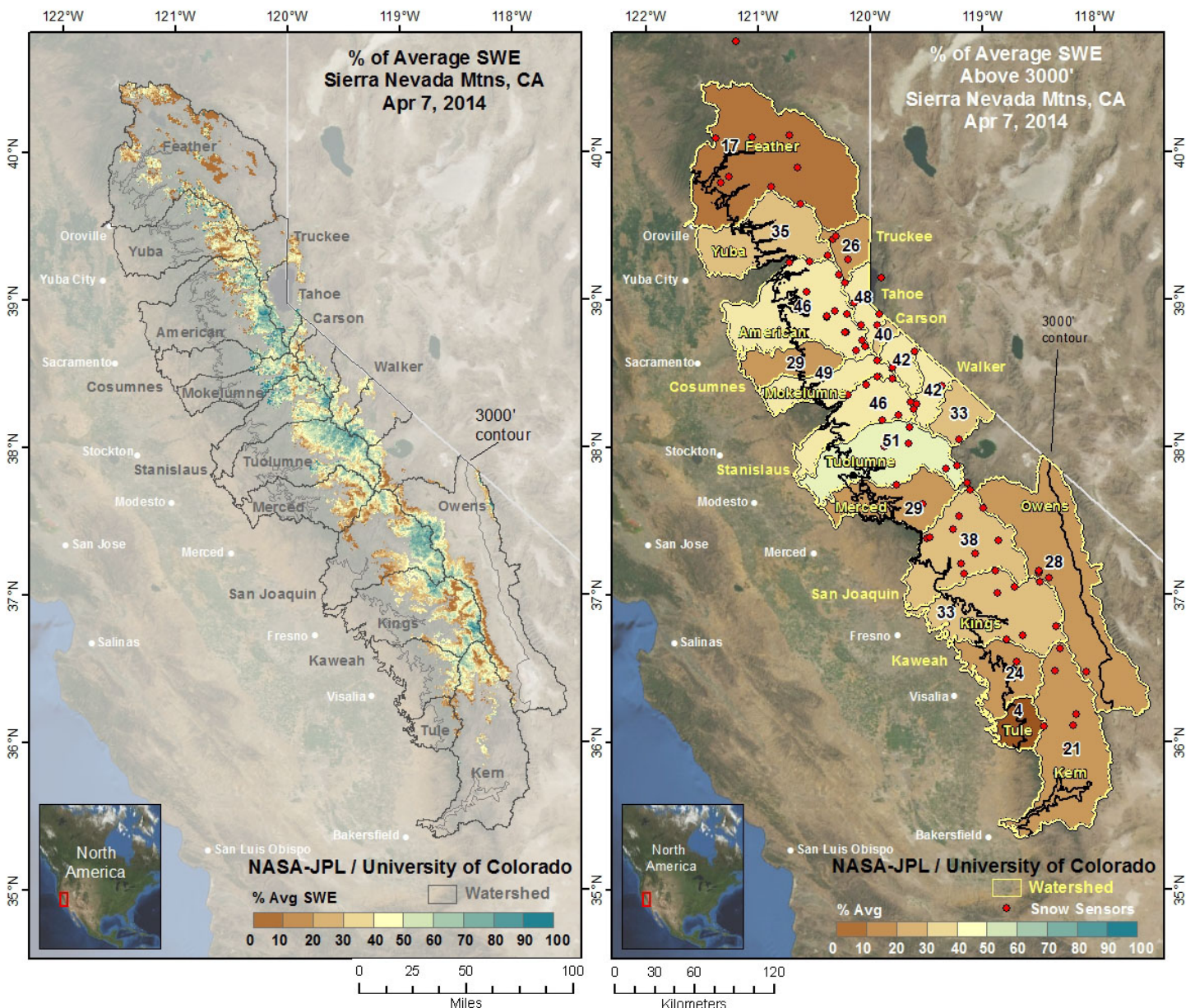
Figure 2. Percent of average RT simulated SWE for April 7, 2014 for the entire Sierra (on left) and by watershed (on right). Watershed percentages are calculated for all model pixels above 3000' (shown as gray line on left map). SWE snow sensors that had snow on April 7, 2014 have been added to the map on the right.
