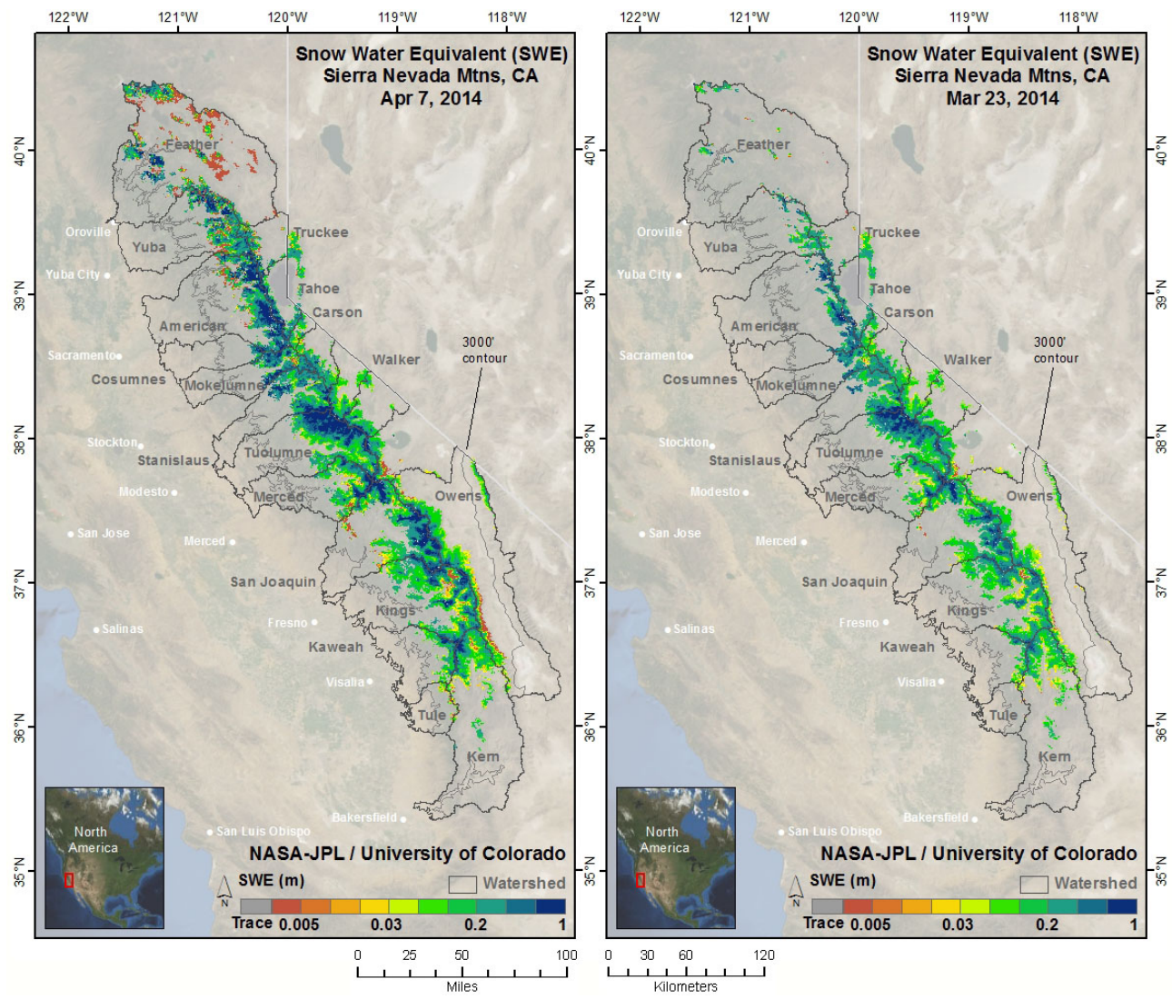
Figure 1. RT simulated SWE amounts for Apr 7, 2014 are shown on the left and for Mar 23, 2014 are shown on the right. SWE depths have increased at all elevations and snow extent has increased since the last report.
