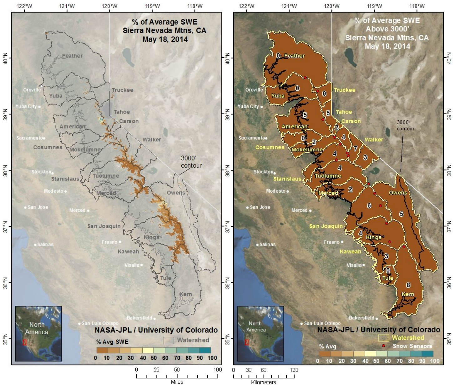
Figure 2. Percent of average RT simulated SWE for May 18, 2014 for the entire Sierra (on left) and by watershed (on right). Watershed percentages are calculated for all model pixels above 3000' (shown as gray line on left map). SWE snow sensors that had snow on May 18, 2014 have been added to the map on the right.
