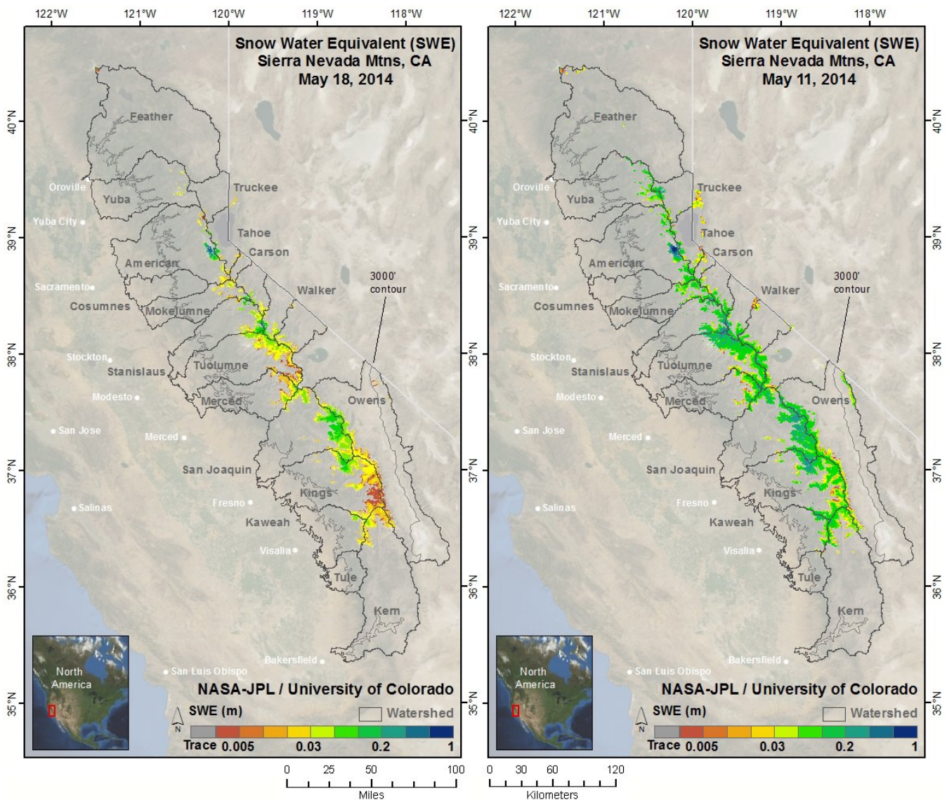
Figure 1. RT simulated SWE amounts for May 18, 2014 are shown on the left and for May 11, 2014 are shown on the right. SWE depths have decreased at all elevations and snow extent has decreased or remained since the last report.
