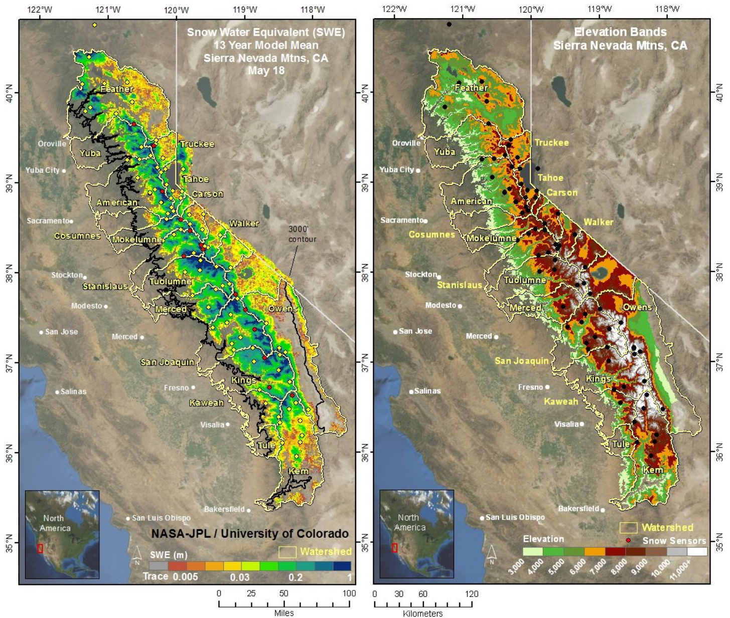
Figure 3. 13 year modeled average SWE for May 18 th on the left with snow sensors shown in yellow that recorded no snow (see discussion above for an explanation) and in red for sensors that recorded snow on May 11, 2014; and a banded elevation map on the right.
