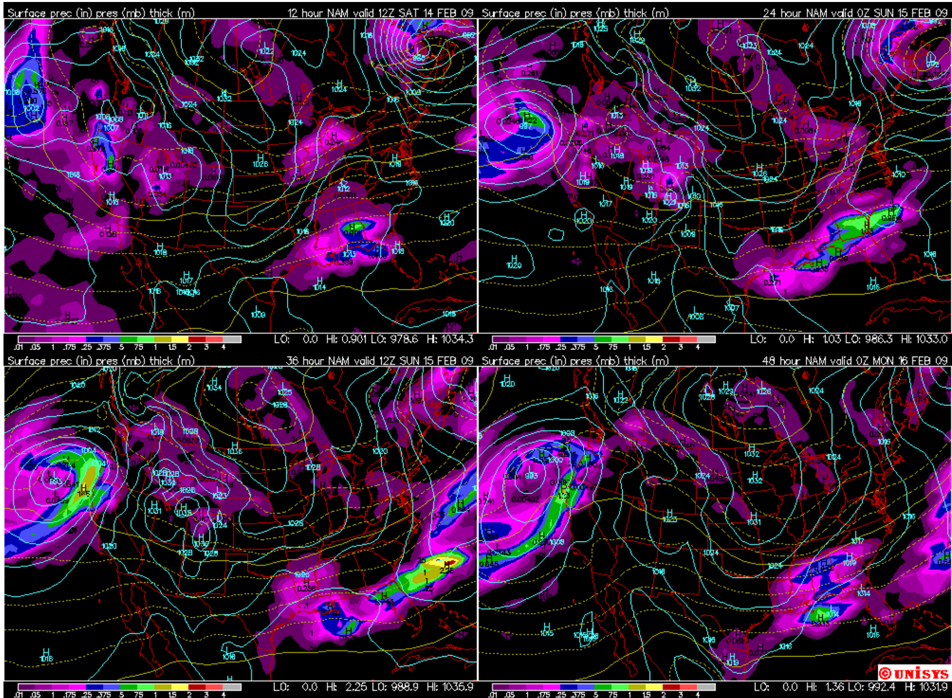
The sea level pressure and precipitation forecast chart includes three parameters: sea level pressure (cyan lines), 1000-500 mb thickness
