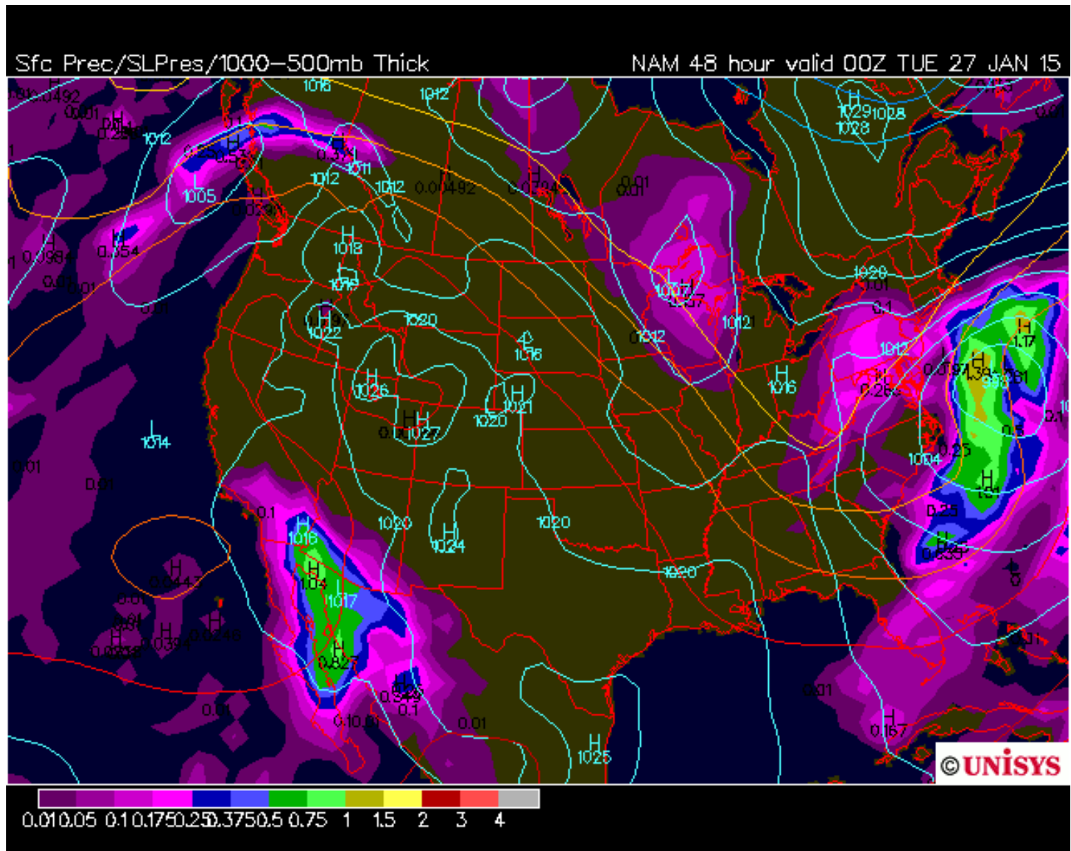
Surface map of pressure (blue lines), temperature (orange to red lines), and precipitation (color bar)
