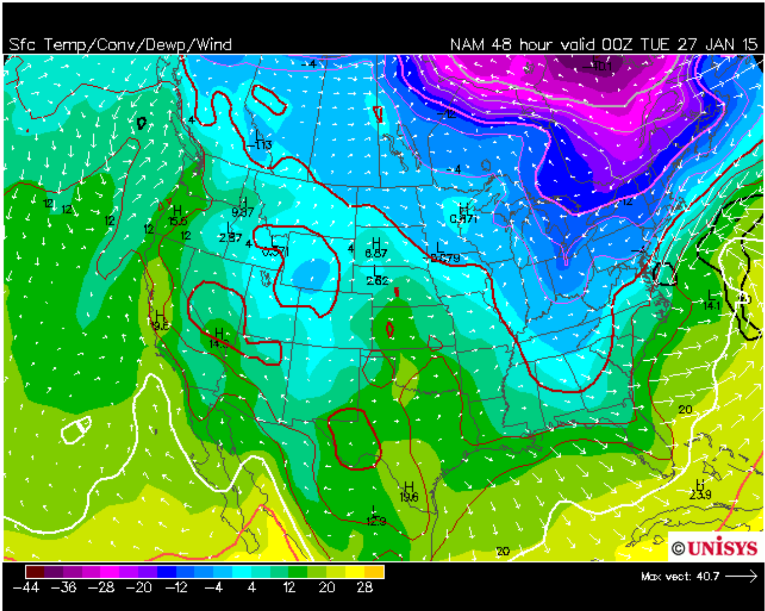
Surface temperature (color bar), Wind (arrows)
