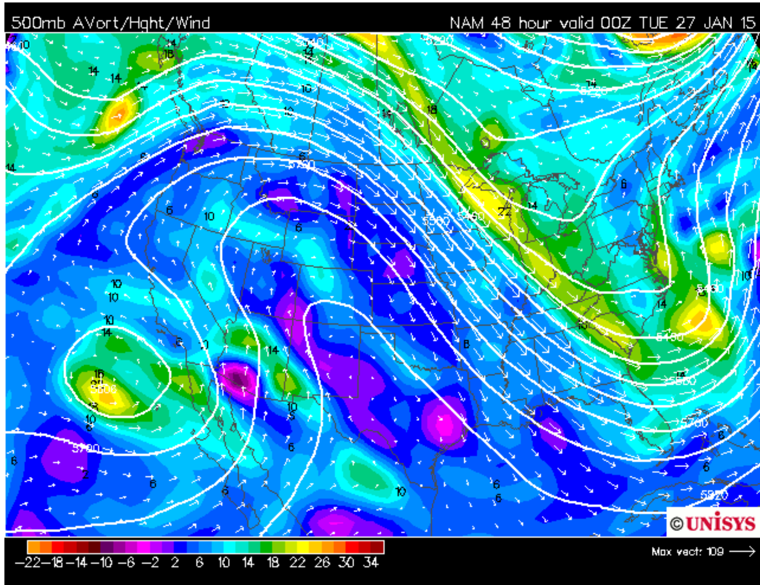
500mb pressure surface (white contours), curvature of pressure lines (color bar), and winds (arrows). Shows the Northern Hemisphere mid-latitude jet over North America. 48-hour forecast is for 00hr UT (=5pm MST Monday 26 Jan 15). On this day, note positions of ridge over western US, and trough over Eastern Seaboard.
