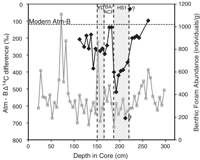
Fig. 3. Comparison of RC27-23 benthic foraminiferal abundances and intermediate water ^{14}\text{C} depletions. Benthic foraminifera abundance data shown in gray open squares are from Anderson (1991). Atmosphere – benthic \Delta^{14}\text{C} differences are shown in black filled diamonds. Atmospheric values are average Intcal09 (Reimer et al., 2009) values for the time interval surrounding each calendar age \pm the calendar age errors. The modern Atmosphere – benthic \Delta^{14}\text{C} difference for \sim 800 m in the Arabian Sea is indicated by a dashed line. Benthic \Delta^{14}\text{C} values determined to be anomalous (see Section 4.1) are indicated by question marks. YD, BA, ACR and HS1 indicate the Younger Dryas, Bølling-Allerød, Antarctic Cold Reversal and Heinrich Stadial 1 intervals respectively.
