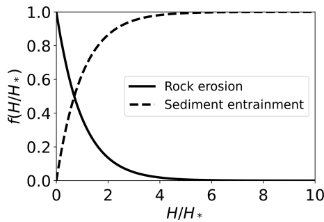
Figure 2. Relative efficiency of fluvial sediment entrainment and bedrock erosion, f(H/H_*) , as a function of the ratio of sediment thickness to bedrock roughness H/H_* . f(H/H_*) depends only on the ratio H/H_* , varies between 0 and 1, and indicates the proportion of total stream power used to entrain sediment – see Eq. 3; f(H/H_*) = 1 - e^{-H/H_*} (dashed line) – or erode bedrock – see Eq. 4; f(H/H_*) = e^{-H/H_*} (solid line). As sediment thickness H increases relative to the bedrock roughness length scale H_* , the sediment entrainment rate factor approaches 1 and the bedrock erosion rate factor approaches 0 because the bed becomes composed entirely of sediment, and no bedrock is exposed. As sediment thickness declines relative to the bedrock roughness length scale, the bedrock erosion rate increases exponentially because more bedrock is exposed, and the sediment entrainment rate declines exponentially due to a lack of available sediment. This approach implements the “cover effect”, in which the presence of sediment reduces bedrock erosion rates but does not incorporate the “tools effect”, in which mobile sediment enhances bedrock erosion. Modified from Shobe et al. (2017).
