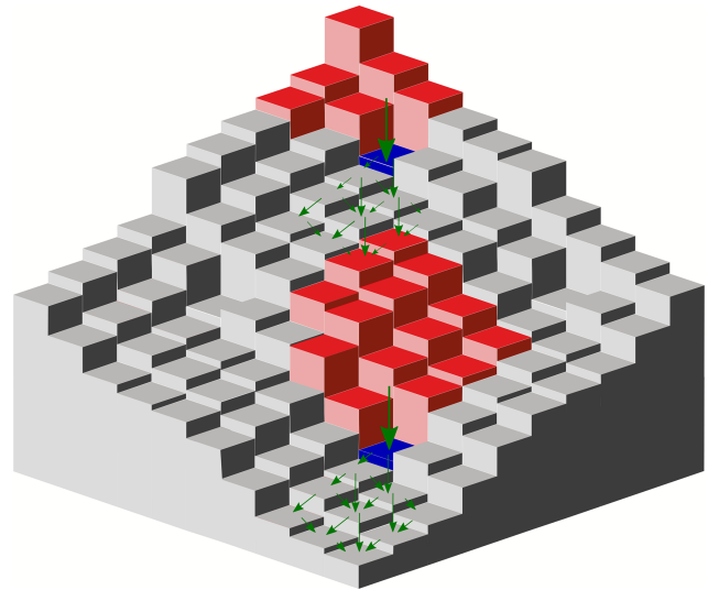
Figure 4. Sketch of landslide algorithm in three dimensions. Cells shaded in blue indicate the critical cells where landslides potentially initiate. Cells shaded in red represent the landslide source areas. After mass failing, sediment will be redistributed over the downslope cells using a multiple-flow-direction algorithm (indicated with green arrows). Sediment deposition rate depends on a transport distance L (see Eqs. 11 and 12).
