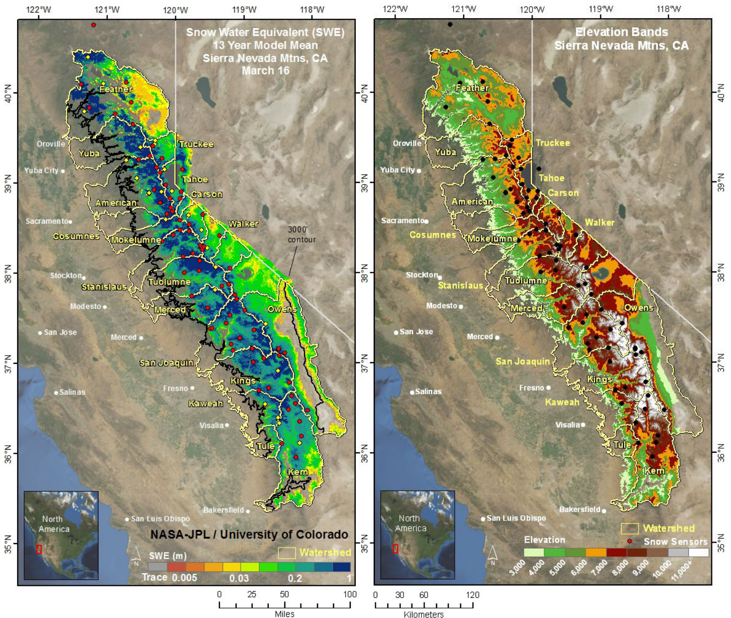
Figure 3. 13 year modeled average SWE for March 16 th on the left with snow sensors shown in yellow that recorded no snow (see discussion above for an explanation) and in red for sensors that recorded snow on March 16, 2014; and a banded elevation map on the right.
