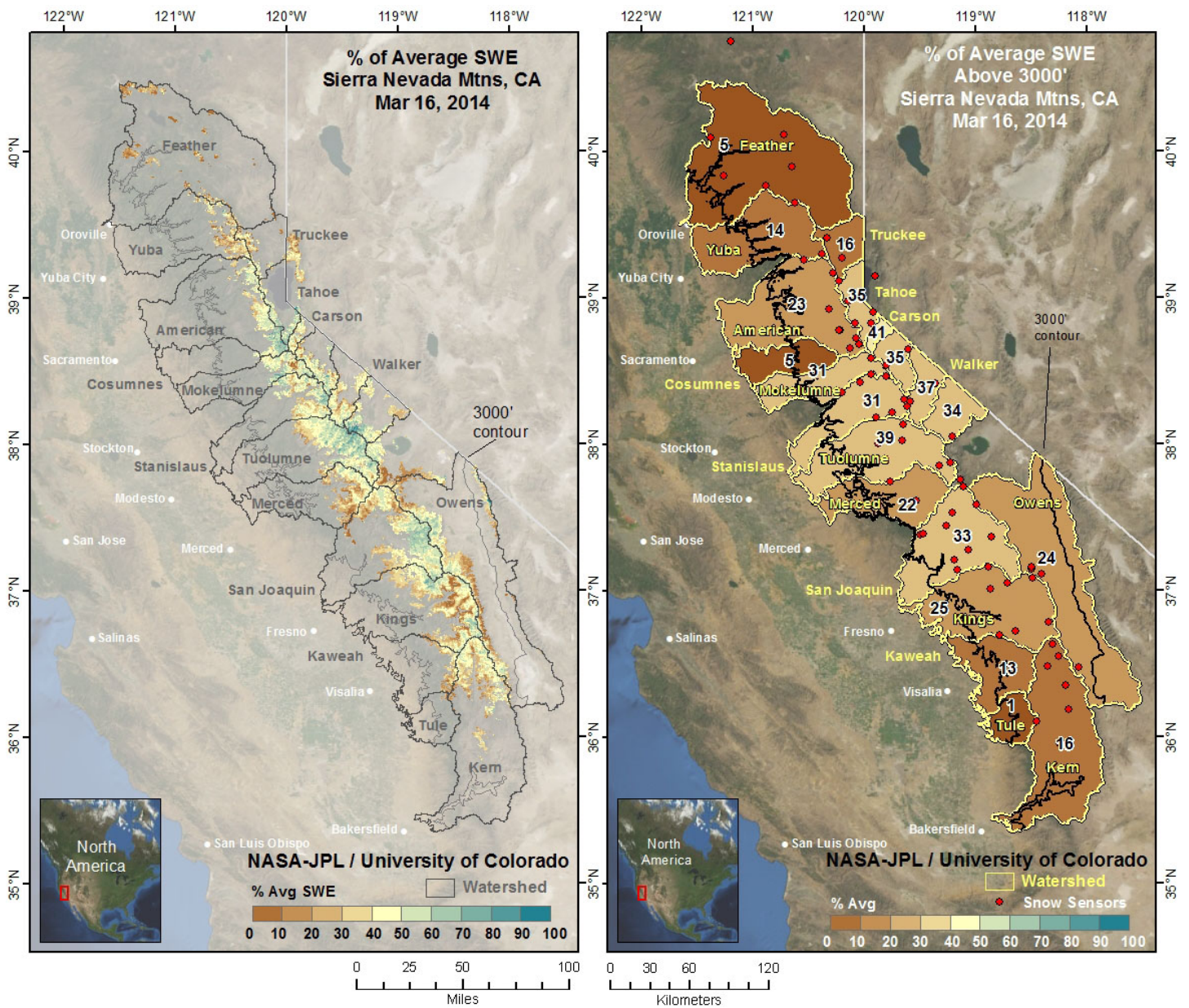
Figure 2. Percent of average RT simulated SWE for March 16, 2014 for the entire Sierra (on left) and by watershed (on right). Watershed percentages are calculated for all model pixels above 3000' (shown as gray line on left map). SWE snow sensors that had snow on March 16, 2014 have been added to the map on the right.
