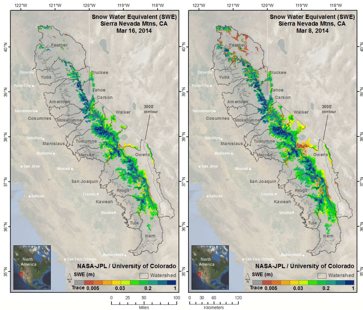
Figure 1. RT simulated SWE amounts for Mar 16, 2014 are shown on the left and for Mar 8, 2014 are shown on the right. SWE depths have decreased at all elevations and snow extent has decreased since the last report.
