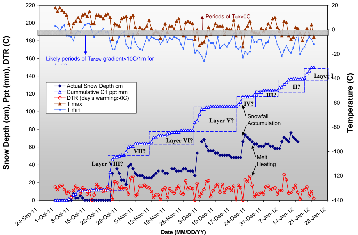
C1 Accumulated Precipitation and Snotel Snowpack Depth / Air Temperature
